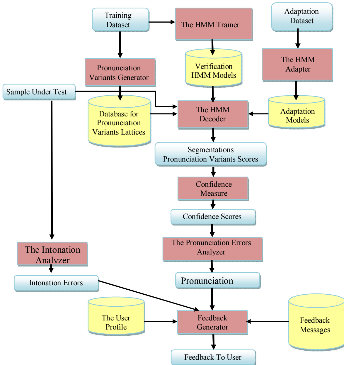
Figure 1: The SpeakCorrect System Architecture
